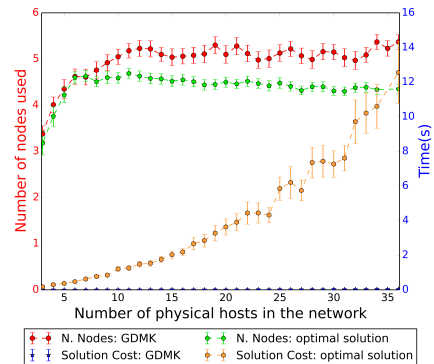
Fig. 5: Varying the number of physical hosts from 1 to 36.
