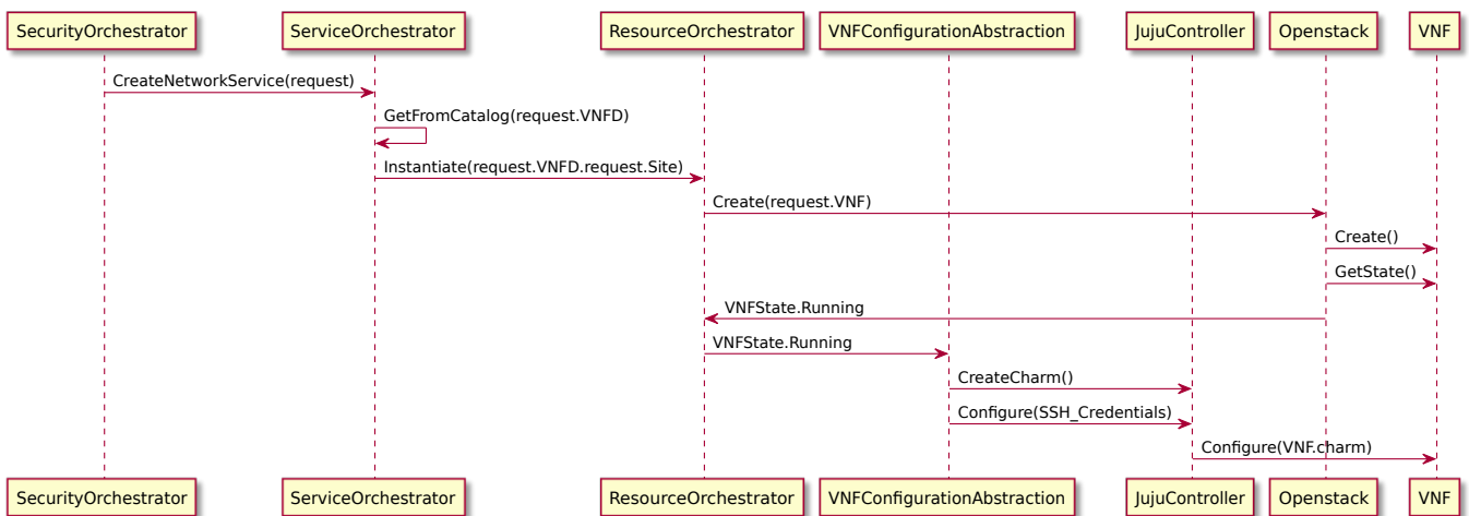
FIGURE 5 VNF Instantiation and Configuration with NFV MANO
