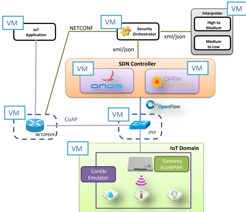
FIGURE 6 Virtual Testbed Deployment
