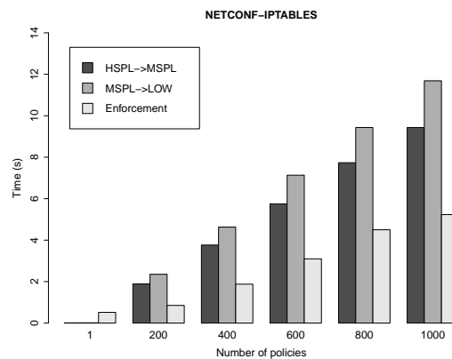
FIGURE 9 Testbed Results. Enforcement with classical IpTables
