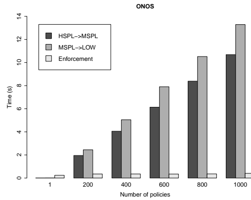
FIGURE 8 Testbed Results. Enforcement with ONOS.
