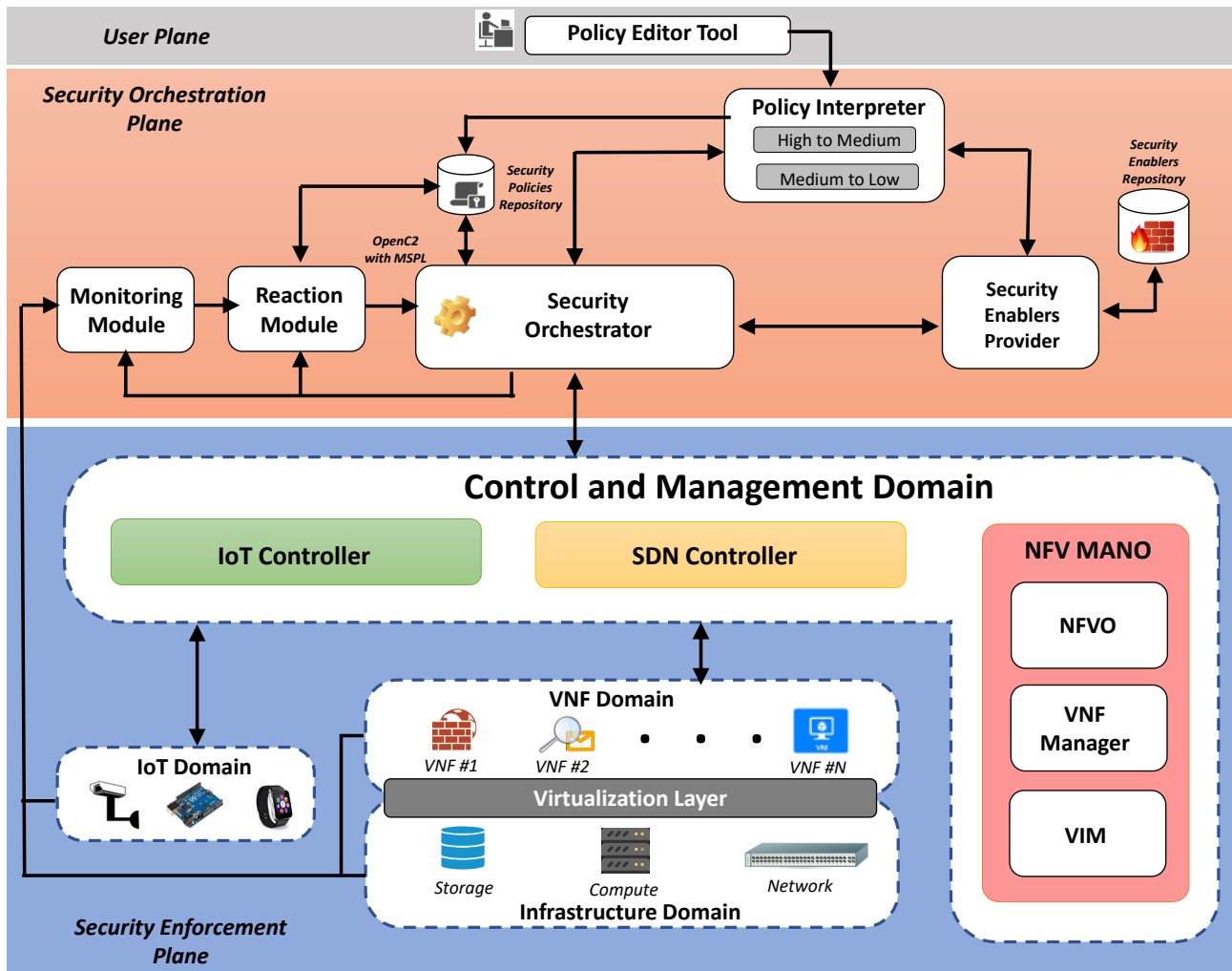
FIGURE 1 Architecture high level overview.
