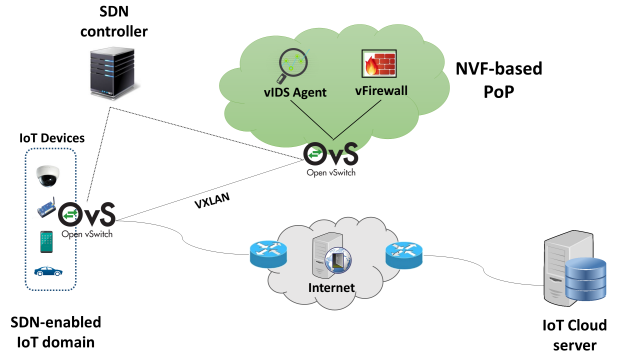
Fig. 10. SDN-based chaining of virtual security functions for IoT environments.
