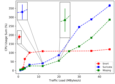
(c) CPU Usage of Snort, Suricata, and Ntopng on the Medium VM.
