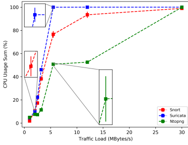
(a) CPU Usage of Snort, Suricata, and Ntopng on the Mini VM.
