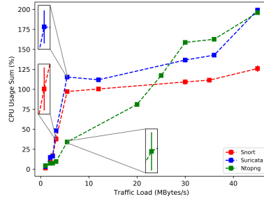
(b) CPU Usage of Snort, Suricata, and Ntopng on the Small VM.
