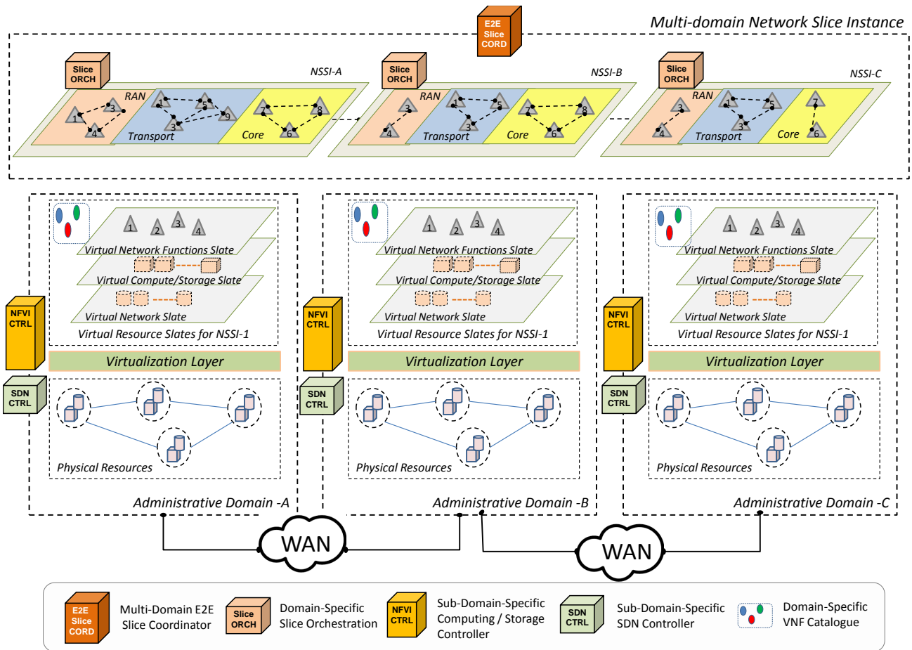
Figure 2: Federated Network Slice Across Multiple Administrative Domains
